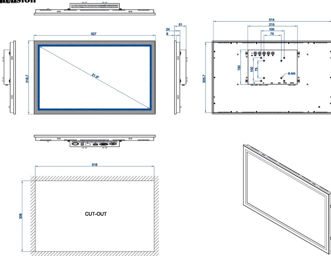
DIMENSIONAL DRAWING:TM-PR215
